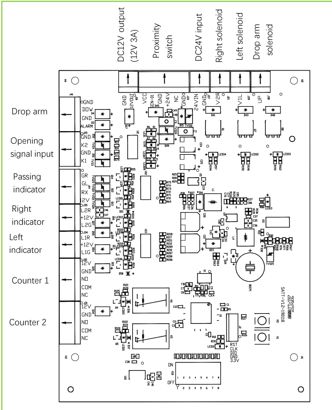
Turnstile control board's diagram as shown in Figure3-1
